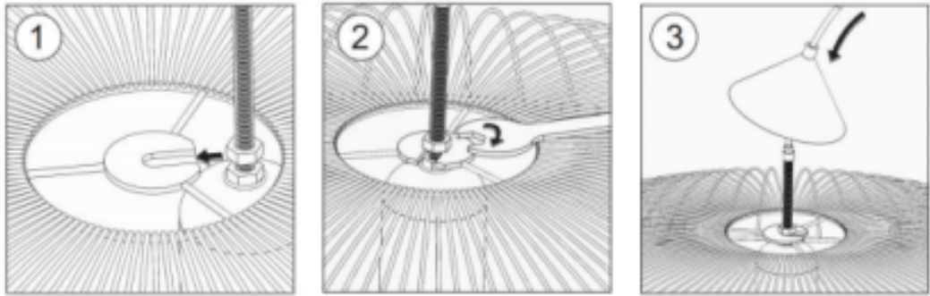
FR / 1. Encastrer la tige filetée ENG / 1. Embed the threaded rod
