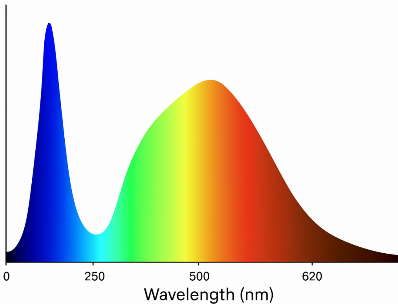
Spectral Power Distribution in the range 250 nm to 800 nm, at full-load
