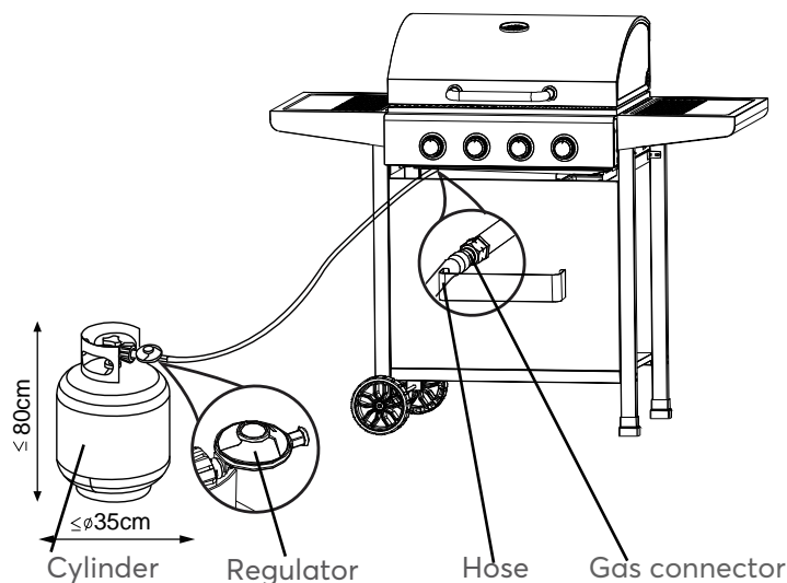
Illustration for the connection of Gas Cylinder, Regulator and Hose
