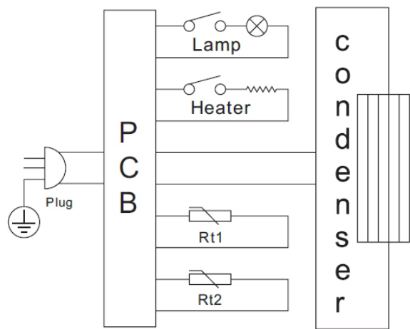
Circuit Diagram
